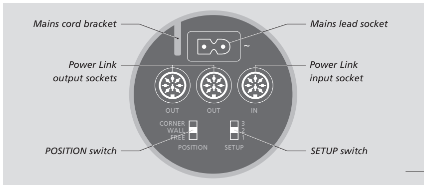
Rear view of BeoLab 2 showing the location of the socket and switch panel.
